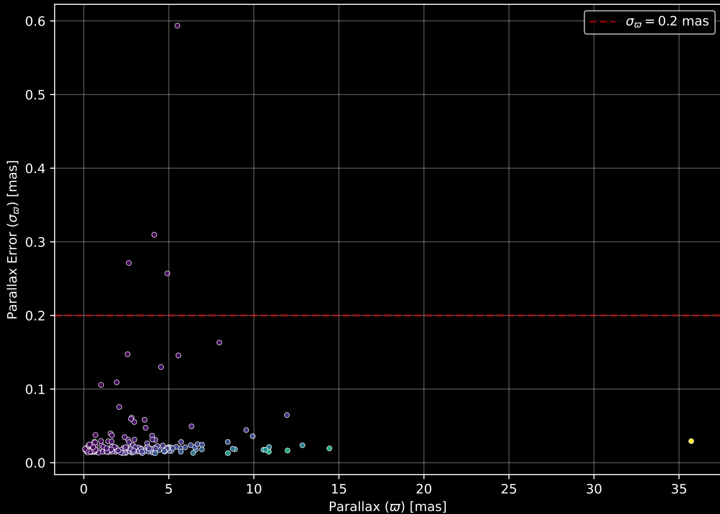
APOGEE DR17 Field: [337+63_MGA] Parallax Quality (n= 183)
