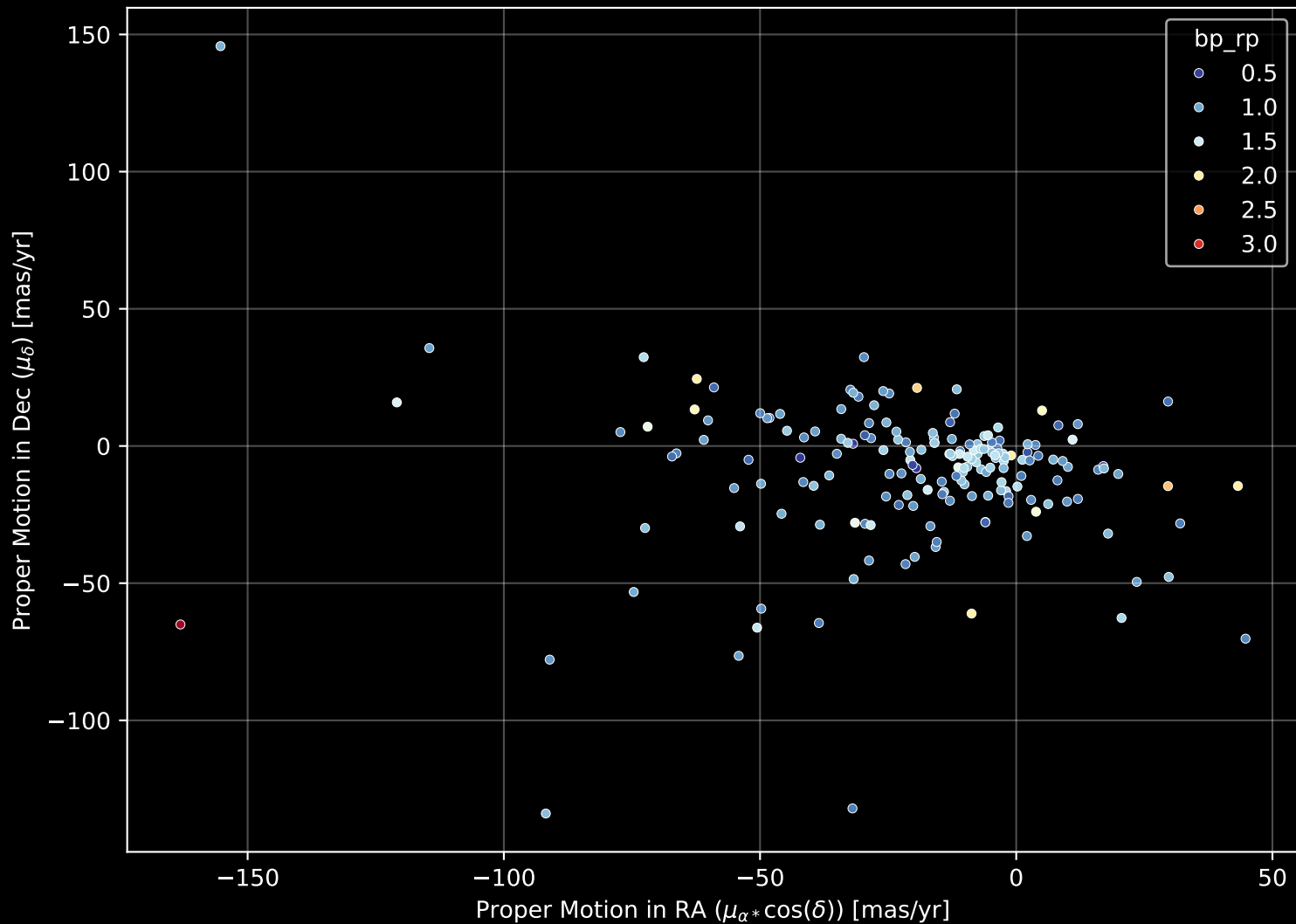
APOGEE DR17 Field: [337+63_MGA] Proper Motion Diagram (n= 183)
