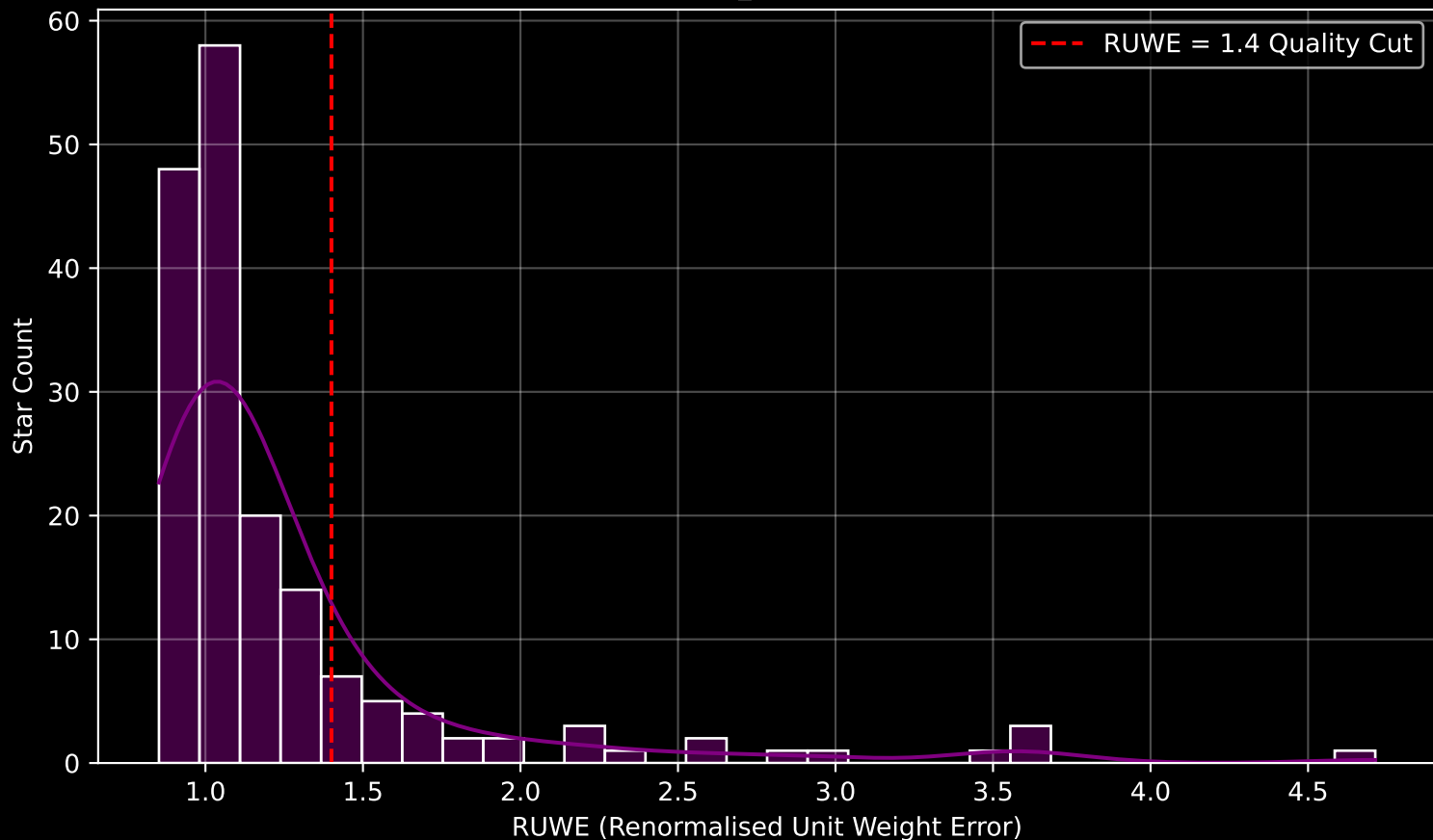
GAPOGEE DR17 Field [337+63_MGA] RUWE Distribution (n= 173)
