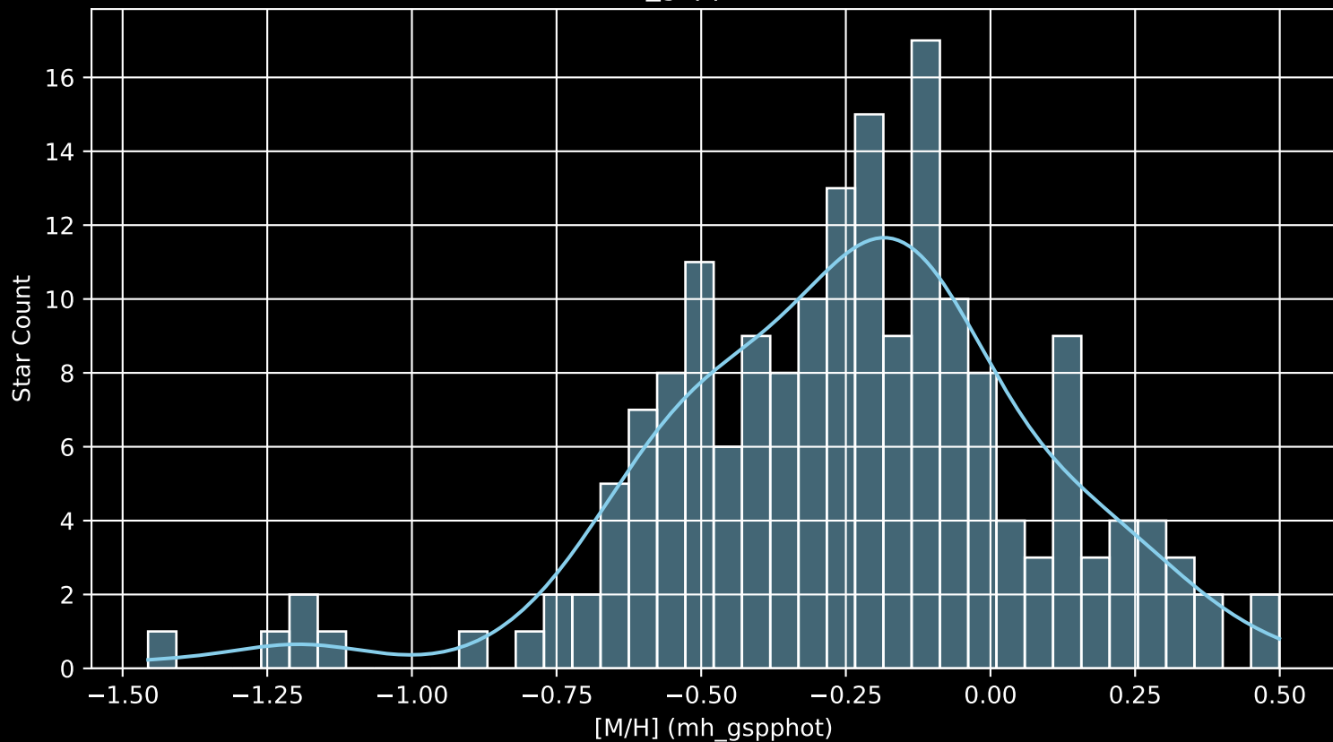
APOGEE DR17 Field: [337+63_MGA [M/H] (mh_gspphot) (n= 181)
