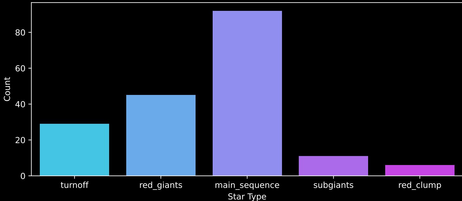
APOGEE DR17 Field: [337+63_MGA] Count plot of Star Type
