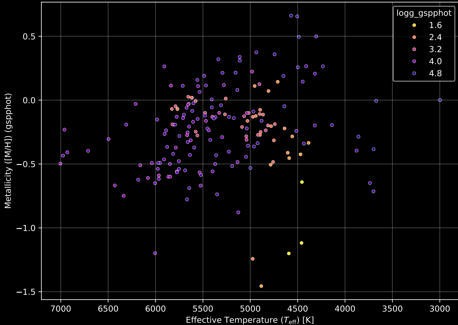
APOGEE DR17 Field: [337+63_MGA] Stellar Population Parameters (n= 183)
